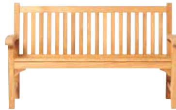
VICTORIA bench w d h kg 125 65 94 22 155 65 94 28 185 65 94 34 215 65 94 40
